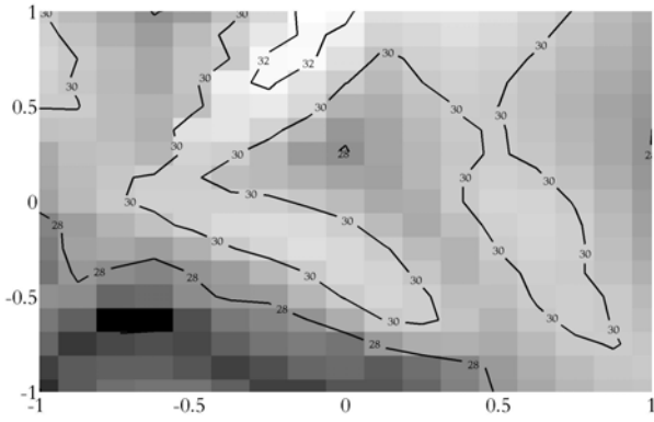
Figure 1. Contours of the maximum value of re-scaled storm peak H_S^* for a typical neighbourhood of locations, N. The background grey-scale is graduated from the lowest (darkest) to the highest (lightest) values per location.
