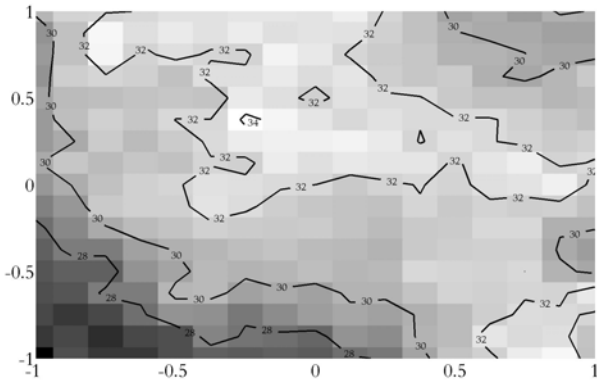
Figure 12. Contours of median re-scaled H_{S100}^* , estimated using the NTPS model on original (un-whitened) data. A [0.5,0.99] quantile whitening band was used with moderate directional smoothing, with a 0.75 quantile threshold for model estimation.
