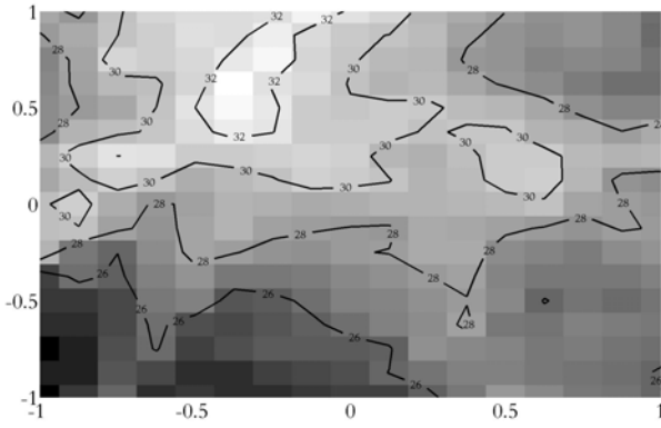
Figure 8. Contours of median re-scaled H_{S100}^* , estimated using the NTPS model on whitened data. A [0.5,0.99] quantile whitening band was used with moderate directional smoothing, with a 0.75 quantile threshold for model estimation.
