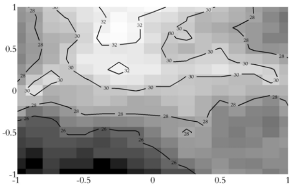
Figure 17. Contours of median re-scaled H_{S100}^* , estimated using the NTPS model on whitened data. A [0.5,0.99] whitening band was used with heavy directional smoothing, with a 0.75 quantile threshold for model estimation. There is reasonable correspondence with Figure 8
