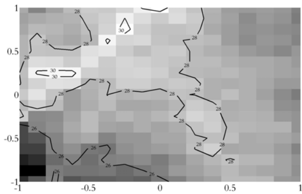
Figure 18. Contours of median re-scaled H_{S100}^* , estimated using the NTPS model on whitened data. A [0.5,0.99] whitening band was used with considerable directional smoothing, with a 0.90 quantile threshold for model estimation. There is reasonable correspondence with Figure 8
