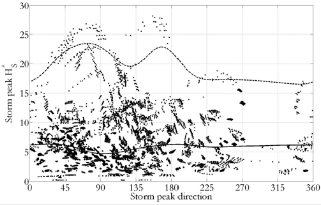
Figure 2. Re-scaled storm peak H_S^* data with storm peak direction for a typical 5 \times 5 grid of neighbouring locations, with estimates of the local median (solid) and 0.99 quantile with respect to direction. There is considerable variation in the values of re-scaled storm peak H_S^* with direction. Storm peak direction gives the direction from which storms emanate, measured clockwise, with North at 0 degrees.
