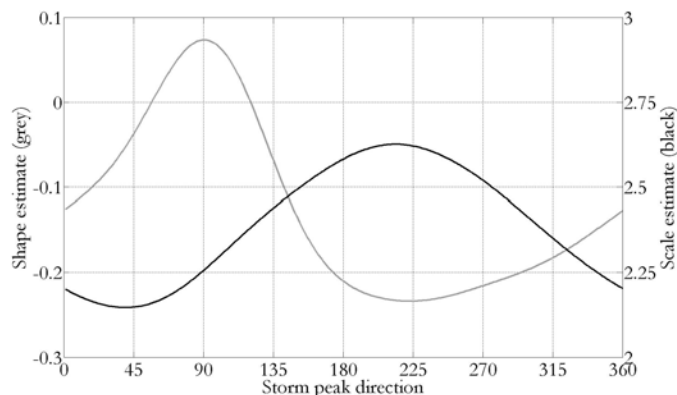
Figure 15. Estimates for generalised Pareto shape (grey) and scale (black) at location L .
