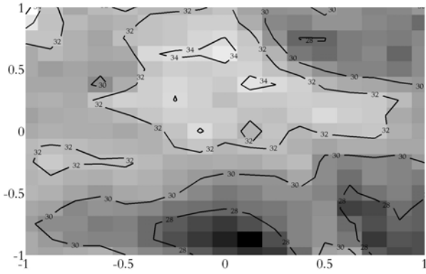
Figure 16. Contours of median re-scaled H_{S100}^* , estimated using the NTPS model on whitened data. A [0.5,0.9] whitening band was used with moderate directional smoothing, with a 0.75 quantile threshold for model estimation. There is reasonable correspondence with Figure 8
