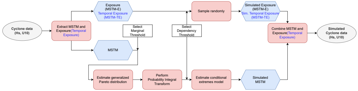
Figure 2: A diagrammatic overview of MSTM-E and MSTM-TE estimation procedures. Red boxes are actions, and blue boxes are data. Blue text denotes actions or data for the MSTM-TE procedure.
