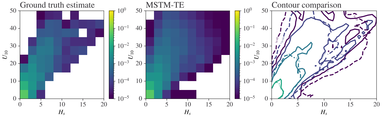
Figure 11: Joint density of sea-state H_S and U_{10} within an extreme tropical cyclone, at reference location 1. The left-hand panel gives the ground truth estimate obtained empirically from the full T_0 = 1,000 years of east cluster TC data for the location. The centre panel shows the estimate obtained under multiple MSTM-TE models, each generated from (randomly-selected) T_S = 200 years of east cluster TC data. The right-hand panel provides a contour plot comparing the empirical ground truth estimate (solid lines) with the MSTM-TE estimates (dashed lines).
