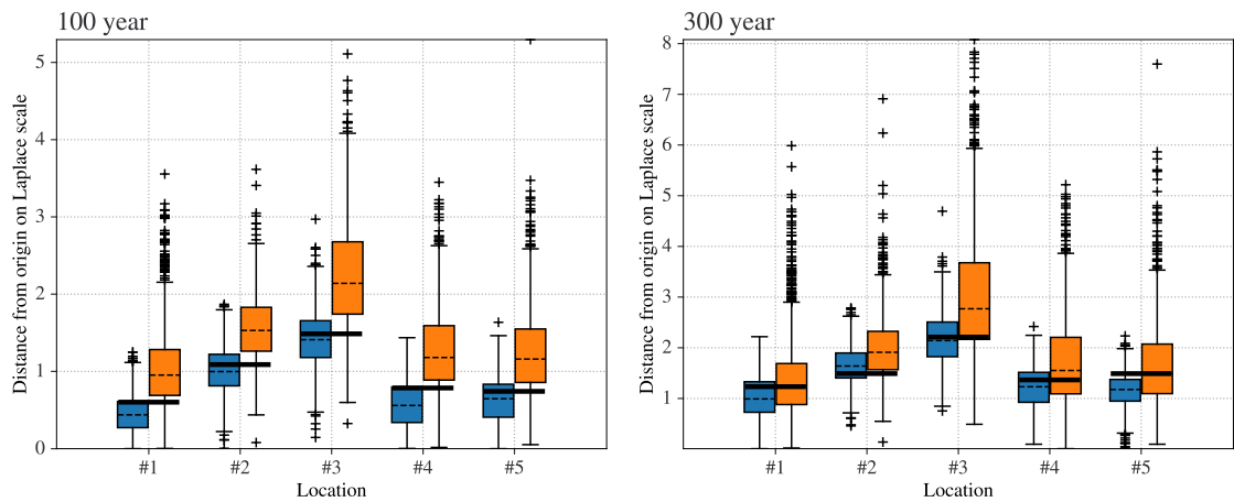
Figure 10: Box-whisker plots comparing contour distances for MSTM-E (blue) and LSE (orange) with empirical ground truth estimates (thick black), for contour return periods T = 100 years (left) and 300 years (right) using east cluster data. The colour scheme follows fig. 8
