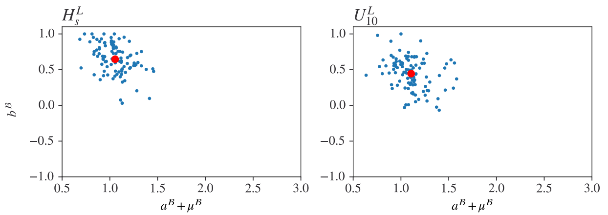
Figure S.5.4: Parameter estimates (a^B + \mu^B, b^B) from 100 bootstrap resamples, and their mean (\hat{a}^B + \hat{\mu}^B, \hat{b}^B) in red for the west cluster.
