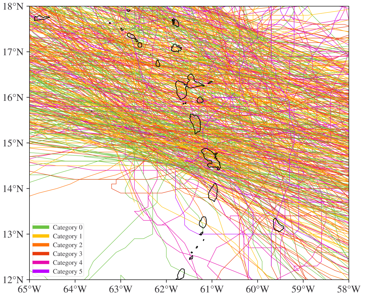
Figure S.2.4: The 685 tracks of cyclones, grouped by its TC intensity category (using Saffir-Simpson scale).
