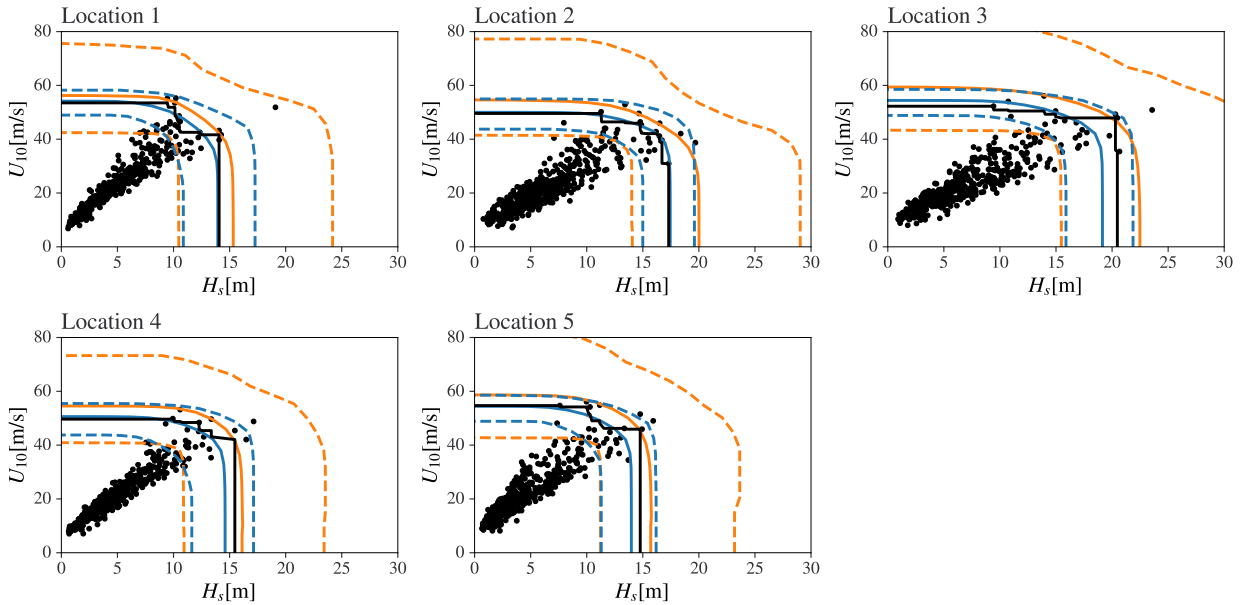
Figure 9: Environmental contours for return period T = 300 years at each of reference locations 1-5, using east cluster data. For full description, see fig. 8.
