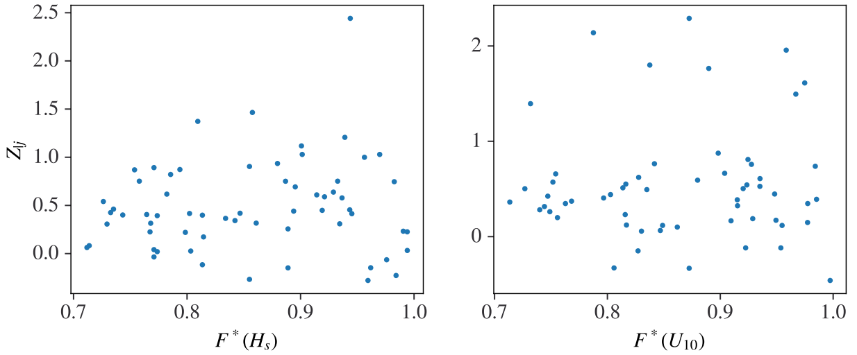
Figure S.3.10: Residual Z_{ij} against the conditioning variable (in uniform margins) for the west cluster.
