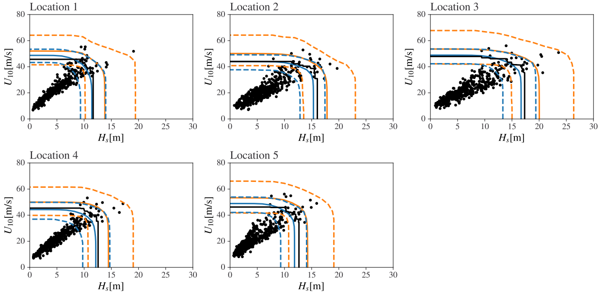
Figure 8: Environmental contours for return period T = 100 years at each of reference locations 1-5, using east cluster data. In each panel, black points represent temporal maxima for TCs at the location. Coloured lines correspond to contours estimated empirically (black), using MSTM-E (blue), and using LSE (orange) respectively. Solid lines give median contours over random selections of 200 years of training data (see section 3.8.1), and dashed lines corresponding central 95% uncertainty intervals. Empirical ground truth estimates are obtained from the full 1,000 years of east cluster TC data for the location of interest.
