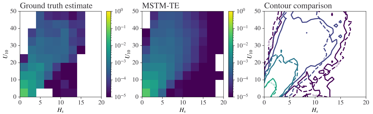
Figure S.8.2: (Location 2) The probability density of the original samples and the samples simulated using MSTM-TE
