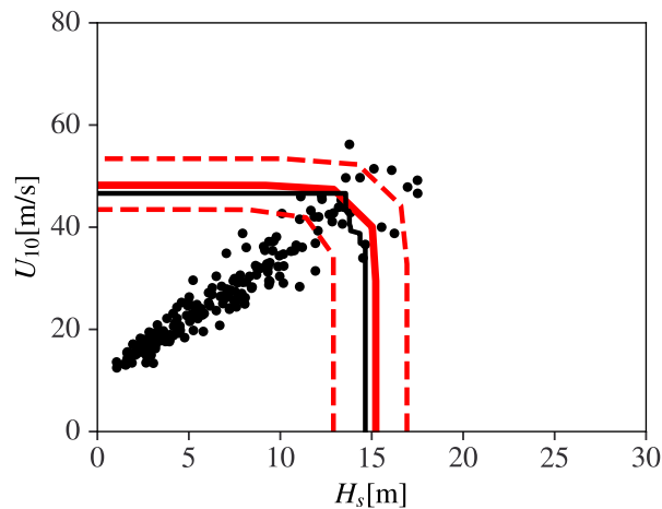
Figure S.6.2: 100-year RV of MSTM for the west cluster. To be compared with fig. 6.
