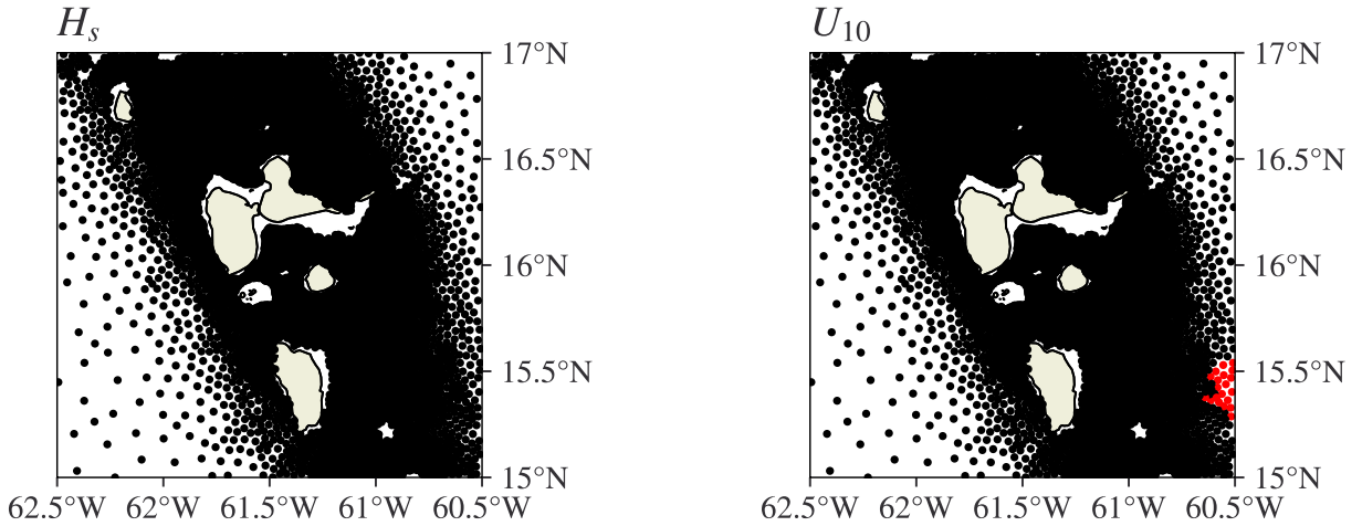
Figure S.4.2: Kendall's tau test at each location for the west cluster. Red points are locations where the p-value is below 0.05, which indicate an untrivial correlation between STM and Exposure.
