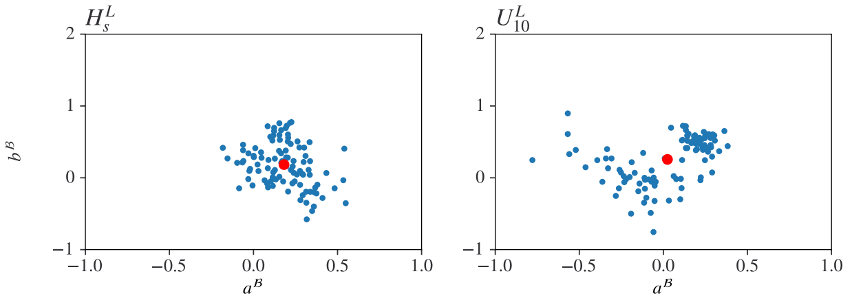
Figure S.5.1: Parameter estimates (a^B, b^B) from 100 bootstrap resamples, and their mean (\hat{a}^B, \hat{b}^B) in red for the east cluster.
