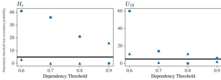
Figure 7: Percentage of locations with non-negligible rank correlations between STM and E for H_S (left) and U_{10} (right), in the west cluster (triangle) and the east cluster (circle), as a function of the non-exceedence probability of the dependence threshold.
