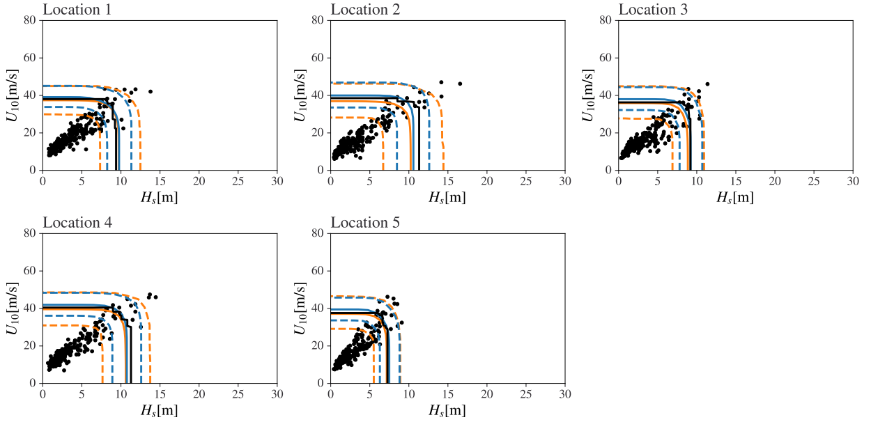
Figure S.6.3: Environmental contours of levels corresponding to 100 year return period for the west cluster. To be compared with fig. 8. We can see that the general size of TCs from the west cluster is smaller than that of TCs from the east cluster. We note also that the number of TCs in the west cluster (218) is smaller than that in the east cluster TCs (467), which would be expected to affect the relative widths of uncertainties for inferences based on the east and west clusters.
