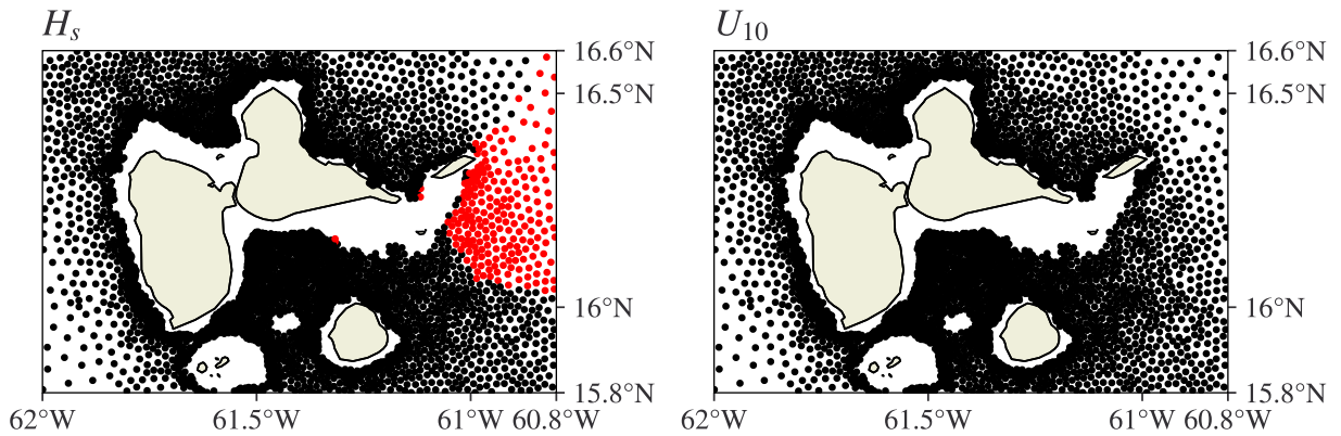
Figure S.7.1: Kendall's tau test for the east cluster in the smaller region selection. Red points are locations where the p-value is below 0.05, which indicate an untrivial correlation between STM and Exposure. To be compared with fig. S.4.1.
