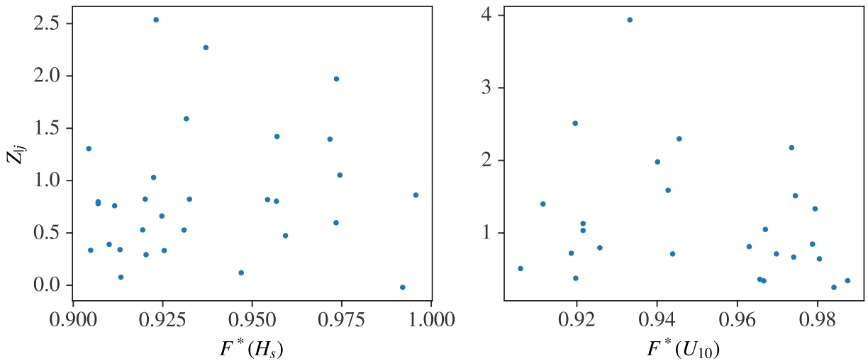
Figure S.3.9: Residual Z_{ij} against the conditioning variable (in uniform margins) for the east cluster.
