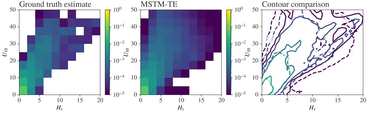
Figure 12: Joint density of sea-state H_S and U_{10} within an extreme tropical cyclone, at reference location 1. The left-hand panel gives the ground truth estimate obtained empirically from the full T_0 = 1,000 years of east cluster TC data for the location. The centre panel shows the estimate obtained under multiple MSTM-TE models, each generated from (randomly-selected) T_S = 200 years of east cluster TC data. The right-hand panel provides a contour plot comparing the empirical ground truth estimate (solid lines) with the MSTM-TE estimates (dashed lines).
