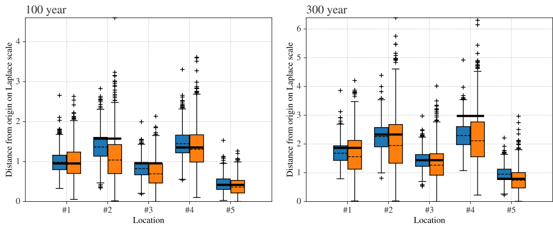
Figure S.6.5: Comparison of return level joint performance for MSTM-E and LSE of different return levels. Color schemes follow fig. 8, with the black bold horizontal lines representing the empirical data. LEFT: Comparison of 100 year return level joint performance for MSTM-E and LSE of the west cluster. RIGHT: Comparison of 300 year return level joint performance for MSTM-E and LSE of the west cluster.
