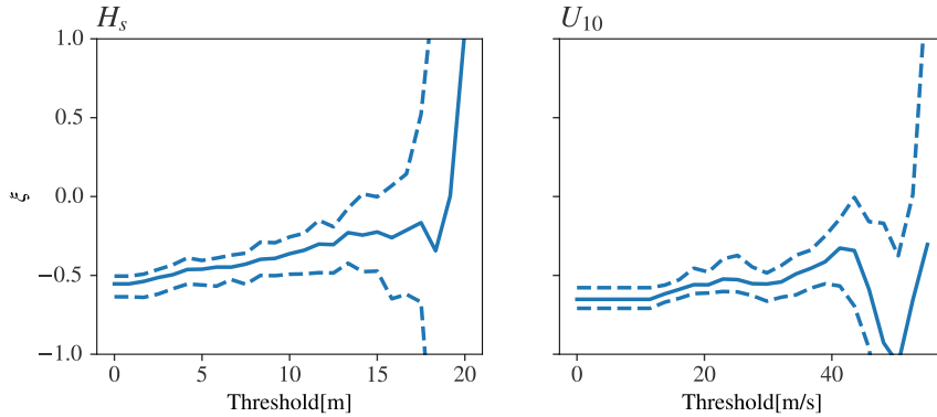
Figure S.3.1: Shape parameter of GP distribution over marginal thresholds for the east cluster. The solid and dashed lines represent the mean and the 2.5-97.5% interval of the bootstrap estimates respectively.
