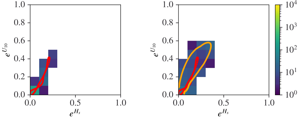
Figure 4: Left: example of a temporal exposure (TE, in red) for an arbitrary choice of TC n and location, in e^{H_S} - e^{U_{10}} space. The cells represent the values of \gamma_n^m(i_1, i_2) , with i_1 and i_2 indicating cell location in discretised H_S and U_{10} respectively. Right: example of TEs (in red and orange) at one location for two TCs n and n' . The cells now represent the values of |\gamma_n^m(i, j) - \gamma_{n'}^m(i, j)| used in eq. (12). Note that the maximum of TEs (red and orange) for each of H_S and U_{10} correspond to exposure E in the corresponding MSTM-E model.
