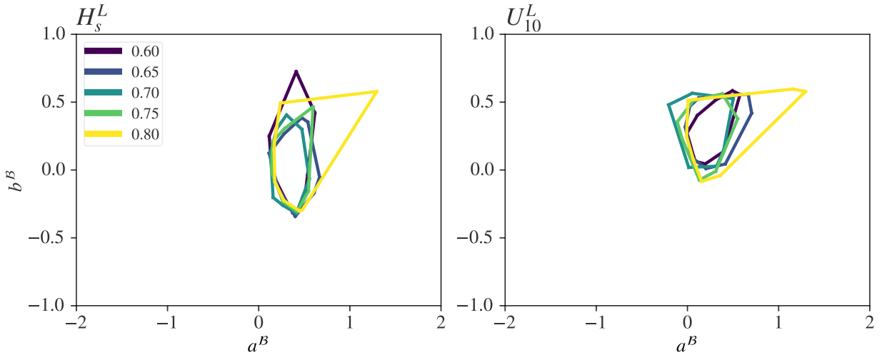
Figure S.3.5: Convex hull of (a^B, b^B) over marginal thresholds with a dependency threshold of 0.6 for the east cluster. As explained in section 3.5, bootstrap mean marginal parameter estimates are used for transformation to standard Laplace scale, and bootstrap resampling then used to estimate the pairs of (a^B, b^B) illustrated in the figure.
