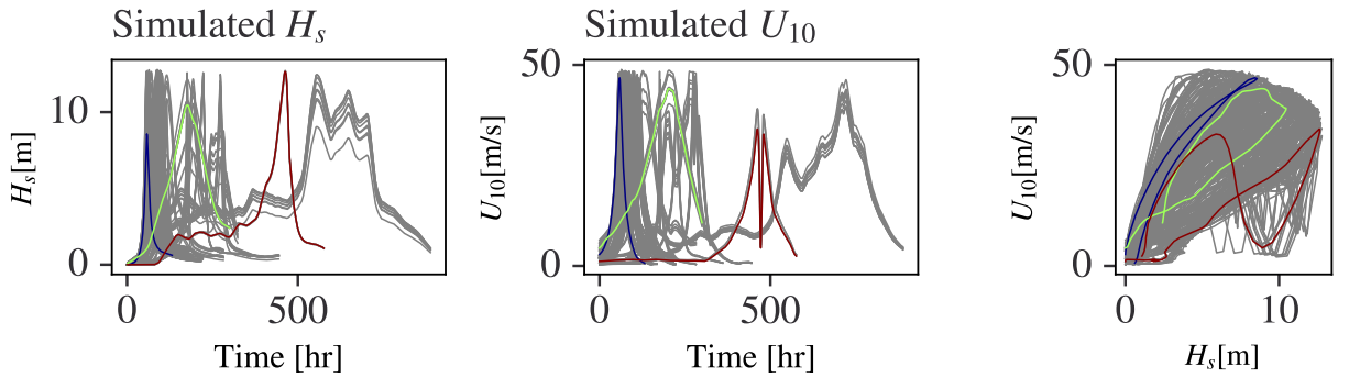
Figure 11: Examples of TC events simulated using MSTM-TE at Location 2. Each line drawn represents the trajectory of a single event, with 3 events coloured (red, green, blue) to illustrate specific instances of the joint evolution of H_S and U_{10} . The left and middle panels show marginal time-series plots of H_S and U_{10} per event, and the right hand panel shows a scatter plot of the joint time-series trajectory in H_S - U_{10} space. Note that events were selected based on MSTM-E (rather than MSTM-TE) H_S, U_{10} values having joint return periods in the interval of 95-105 years. Note further, in the right hand panel, that the boundary created by the set of event trajectories in H_S - U_{10} space resembles the isocontour lines in fig. 8).
