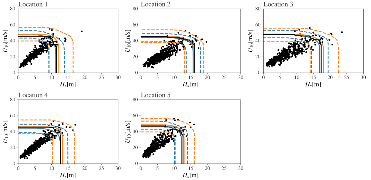
Figure S.7.2: Environmental contours of levels corresponding to 100 year return period for the east cluster in the smaller region selection. To be compared with fig. 8.
