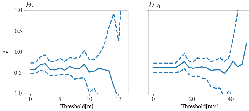
Figure S.3.2: Shape parameter of GP distribution over marginal thresholds for the west cluster. The solid and dashed lines represent the mean and the 2.5-97.5% interval of the bootstrap estimates over ( N_B = 1,000 ) respectively.
