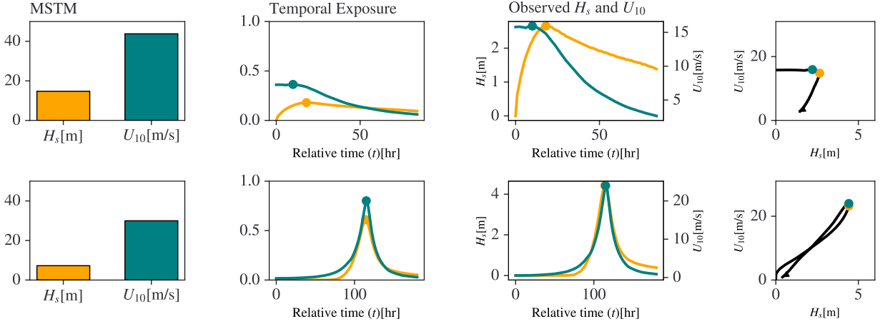
Figure 3: Examples of TC events to aid in understanding MSTM-E and MSTM-TE. Each row of panels correspond to a cyclone event, the track of which is given in fig. 1, with the upper (lower) panel corresponding to the cyclone track in red (orange) in fig. 1. Left to right: the corresponding MSTM (panel 1), TE at location 2 (see fig. 1, panel 2), and the corresponding observed timeseries of (H_S, U_{10}) in time (panel 3) and jointly (panel 4). Note that the maximum TE with respect to H_S and U_{10} for both cyclones is strictly < 1 , indicating that location 2 is not the location of the STM for any combination of metocean variable and cyclone. Note further that TE (panel 2) multiplied by MSTM (panel 1) gives observed time-series (panel 3).
