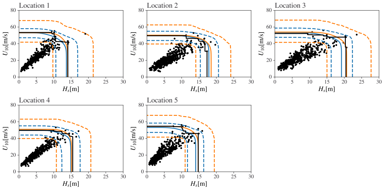
Figure S.7.3: Environmental contours of levels corresponding to 300 year return period for the east cluster in the smaller region selection. To be compared with fig. 9.
