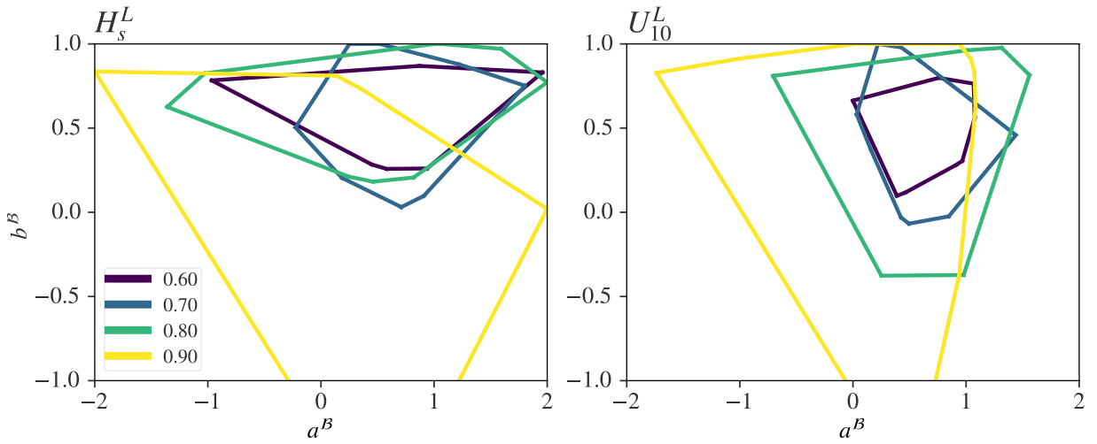
Figure S.3.8: Convex hull of (a, b) over dependency thresholds with a marginal threshold of 0.6 for the west cluster. As explained in section 3.5, bootstrap resampling was used to estimate the pairs of (a, b) .
