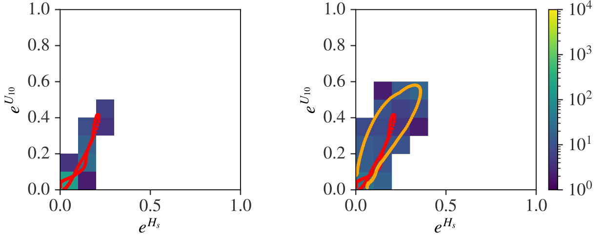
Figure 4: Left: example of a temporal exposure (TE, in red) for an arbitrary choice of TC n and location, in e^{H_S}-e^{U_{10}} space. The cells represent the values of \gamma_n^m(i_1, i_2) , with i_1 and i_2 indicating cell location in discretised H_S and U_{10} respectively. Right: example of TEs (in red and orange) at one location for two TCs n and n' . The cells now represent the values of |\gamma_n^m(i, j) - \gamma_{n'}^m(i, j)| used in eq. (12). Note that the maximum of TEs (red and orange) for each of H_S and U_{10} correspond to exposure E in the corresponding MSTM-E model.
