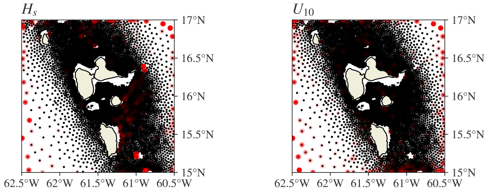
Figure S.2.1: Location of MSTMs (LEFT) H_S , (RIGHT) U_{10} . Color density corresponds to the number of STM occurrences at the location.
