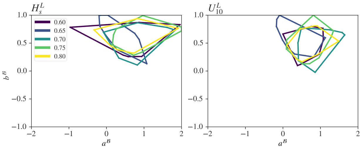
Figure S.3.6: Convex hull of (a, b) over marginal thresholds with a dependency threshold of 0.6 for the west cluster. As explained in section 3.5, bootstrap resampling was used to estimated the pairs of (a, b) .
