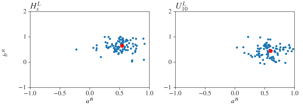
Figure S.5.2: Parameter estimates (a^B, b^B) from 100 bootstrap resamples, and their mean (\hat{a}^B, \hat{b}^B) in red for the west cluster.
