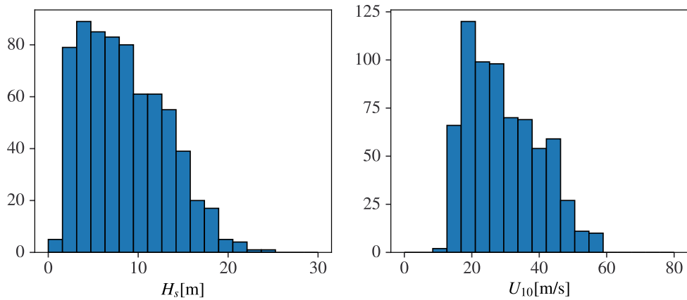
Figure S.2.2: Histogram of MSTM for the Guadeloupe region (60.5-62.5W°, 15.0N-17.0N°) illustrated in fig. 1
