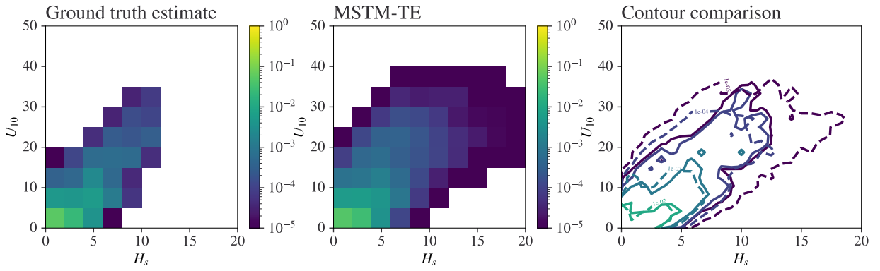
Figure S.8.3: (Location 3) The probability density of the original samples and the samples simulated using MSTM-TE
