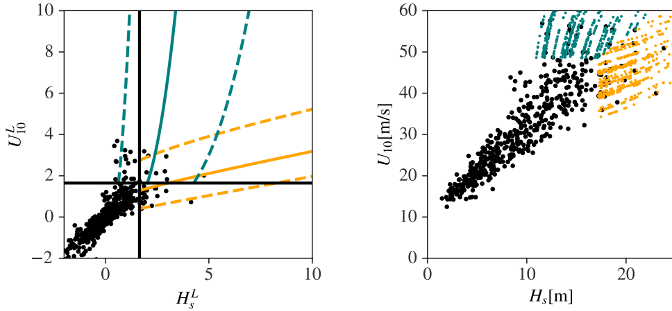
Figure 5: Conditional extreme values models for MSTM in east cluster. Left: conditional models on standard Laplace scale, for U_{10}^L | H_S^L (yellow) and H_S^L | U_{10}^L (blue). Solid lines represent models with bootstrap mean parameter estimates for a , b and \mu . Dashed lines represent 95% uncertainty bands for predictions, estimated using the 2.5% and 97.5% quantiles of the set empirical \mathcal{R} of model residuals Z . Right: conditional model on physical scale. Coloured points represent realisations of MSTM sampled under the fitted models for U_{10} | H_S (yellow) and H_S | U_{10} (blue), together with the original sample (black).
