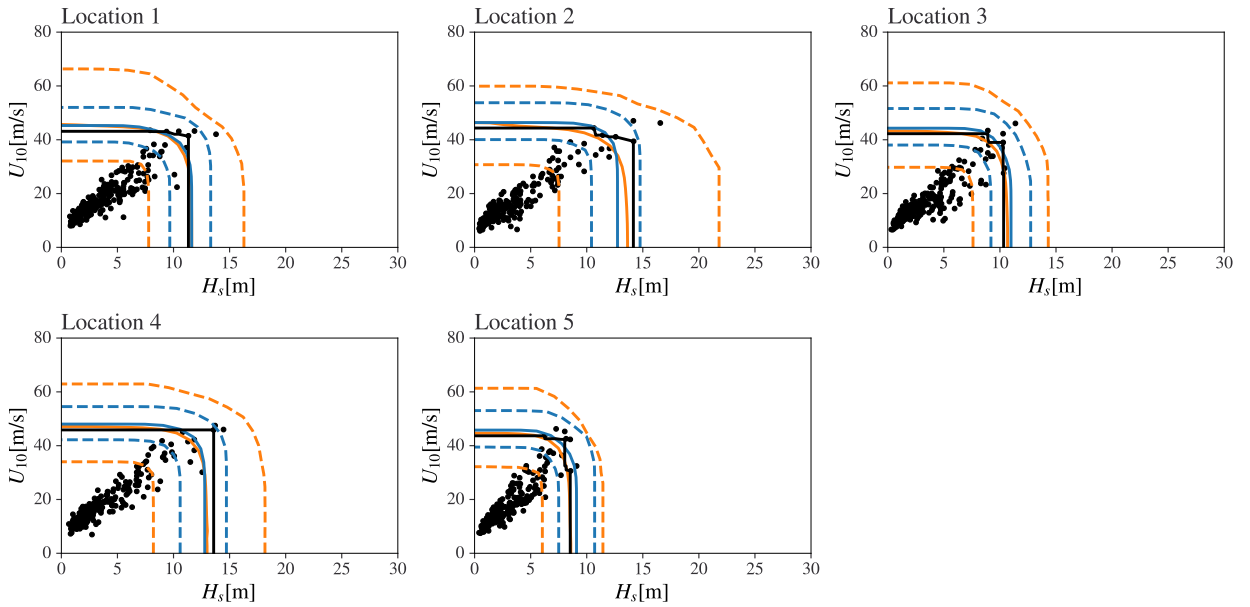
Figure S.6.4: Environmental contours of levels corresponding to 300 year return period for the west cluster. To be compared with fig. 9.
