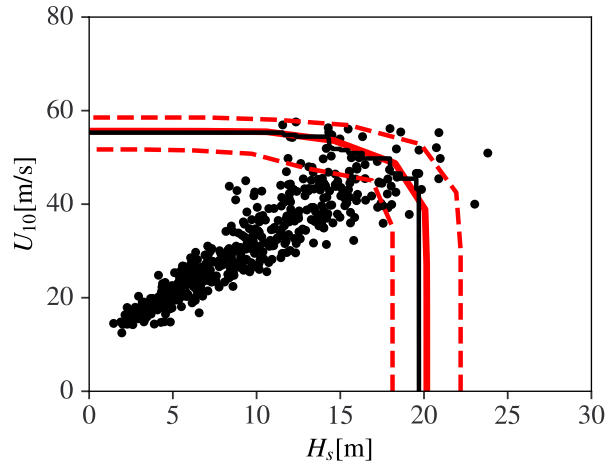
Figure 6: Environmental contours for H_S - U_{10} MSTM of in the east cluster, corresponding to a return period of T = 100 years. The contour estimated under multiple MSTM models given random samples of length T_S = 200 years is shown in red, as a mean contour and its central 95% uncertainty band. The contour shown in black is estimated empirically using the full T_0 = 1,000 years of simulated TC data. The full underlying TC dataset for the east cluster is also shown as black dots.
