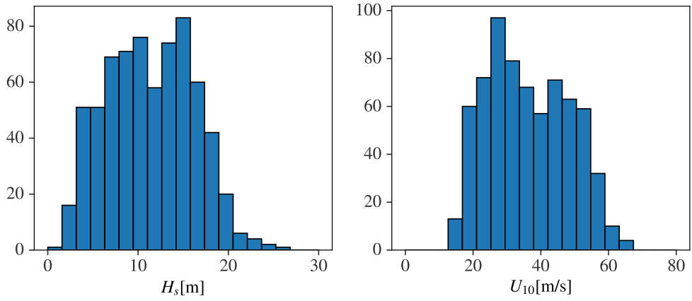
Figure S.2.3: Histogram of STM for the entire region (50.0-84.7W°, 8.4-22.1N°)
