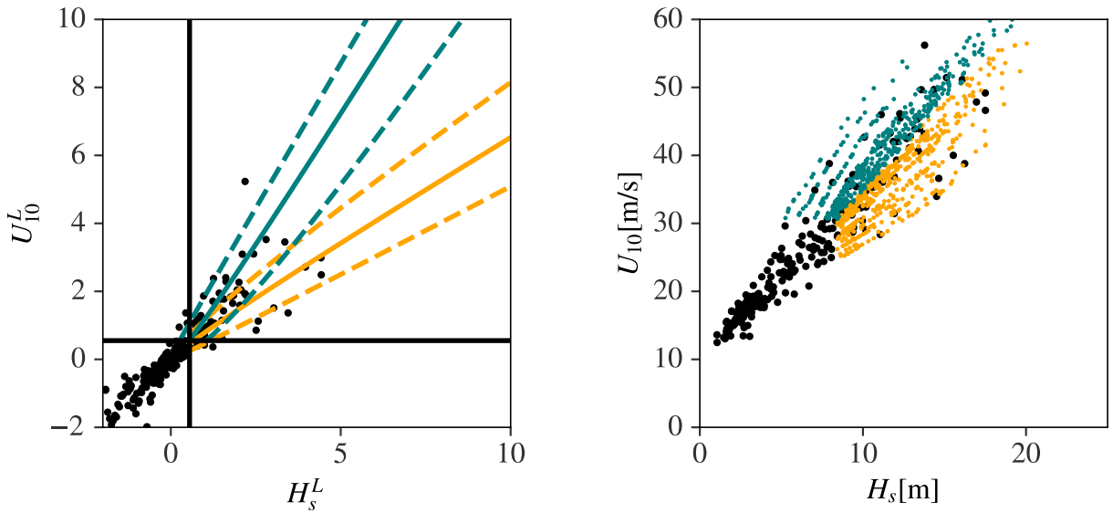
Figure S.6.1: Conditional model of MSTM for west cluster on Laplace scale(left) and in physical scale(right). Dependency threshold is 0.70. To be compared with fig. 5.
