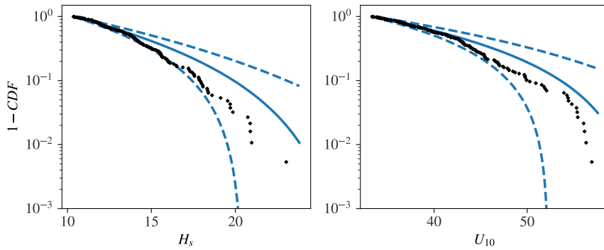
Figure S.3.3: 1-CDF of STM for the bootstrap (blue) and the samples for the east cluster. The solid and dashed lines represent the mean and the 2.5-97.5% interval of the bootstrap estimates ( N = 1,000 ) respectively.
