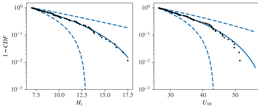
Figure S.3.4: 1-CDF of STM for the bootstrap (blue) and the samples for the west cluster. The solid and dashed lines represent the mean and the 2.5-97.5% interval of the bootstrap estimates ( N = 1,000 ) respectively.
