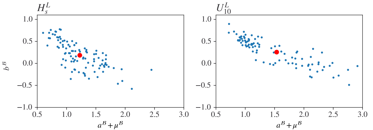
Figure S.5.3: Parameter estimates (a^B + \mu^B, b^B) from 100 bootstrap resamples, and their mean (\hat{a}^B + \hat{\mu}^B, \hat{b}^B) in red for the east cluster.
