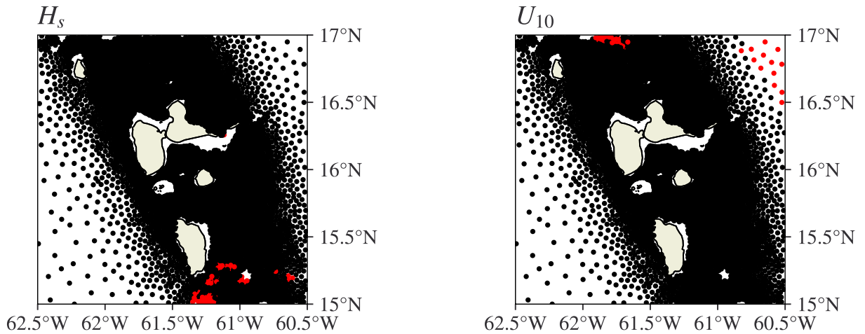
Figure S.4.1: Kendall's tau test at each location for the east cluster. Red points are locations where the p-value is below 0.05, which indicate an untrivial correlation between STM and Exposure.
