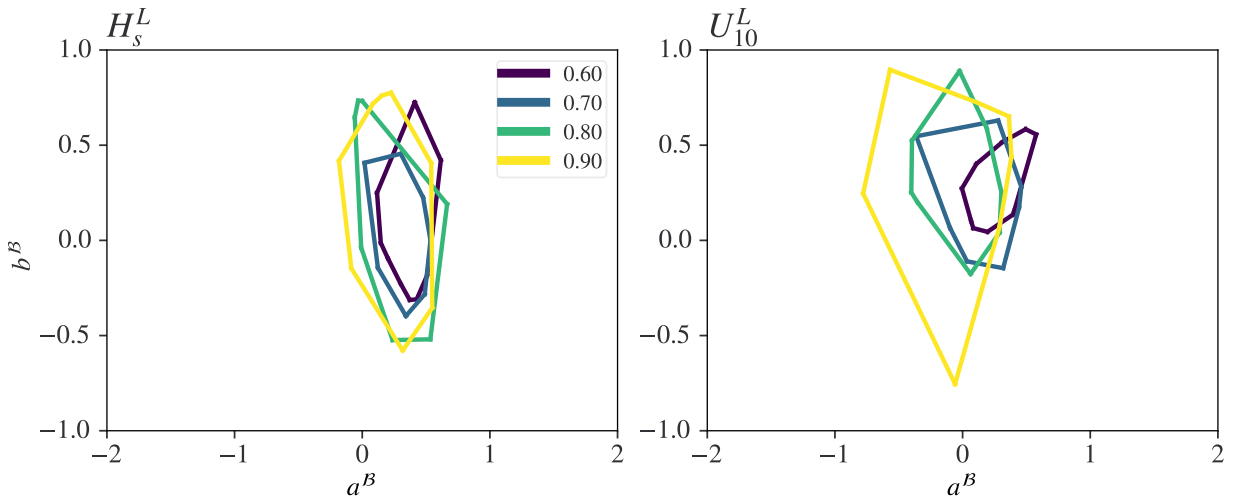
Figure S.3.7: Convex hull of (a, b) over dependency thresholds with a marginal threshold of 0.6 for the east cluster. As explained in section 3.5, bootstrap resampling was used to estimate the pairs of (a, b) .
