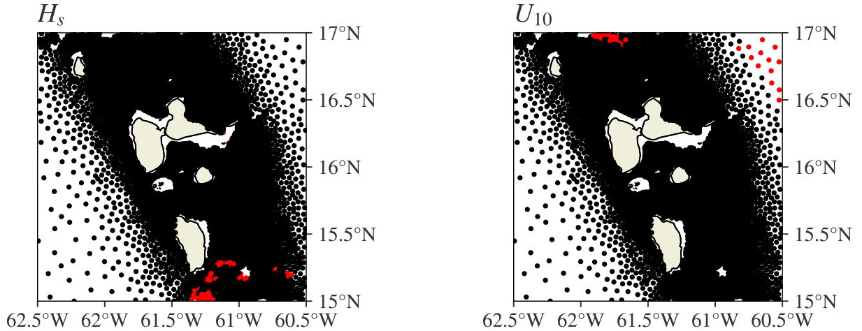
Figure S.8.1: Kendall's tau test for MSTM-TE for the east cluster. Red points are locations where the p-value is below 0.05, which indicate an untrivial correlation between STM and Exposure.
