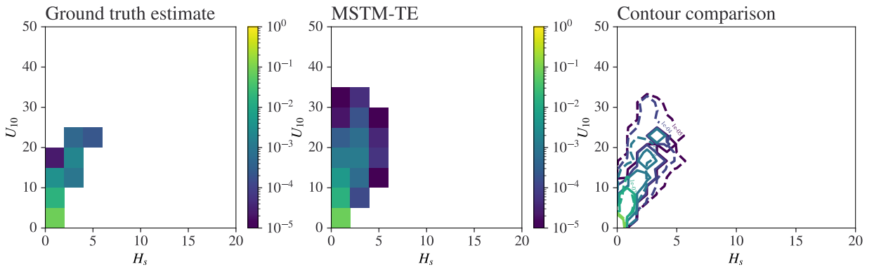
Figure S.8.5: (Location 5) The probability density of the original samples and the samples simulated using MSTM-TE
