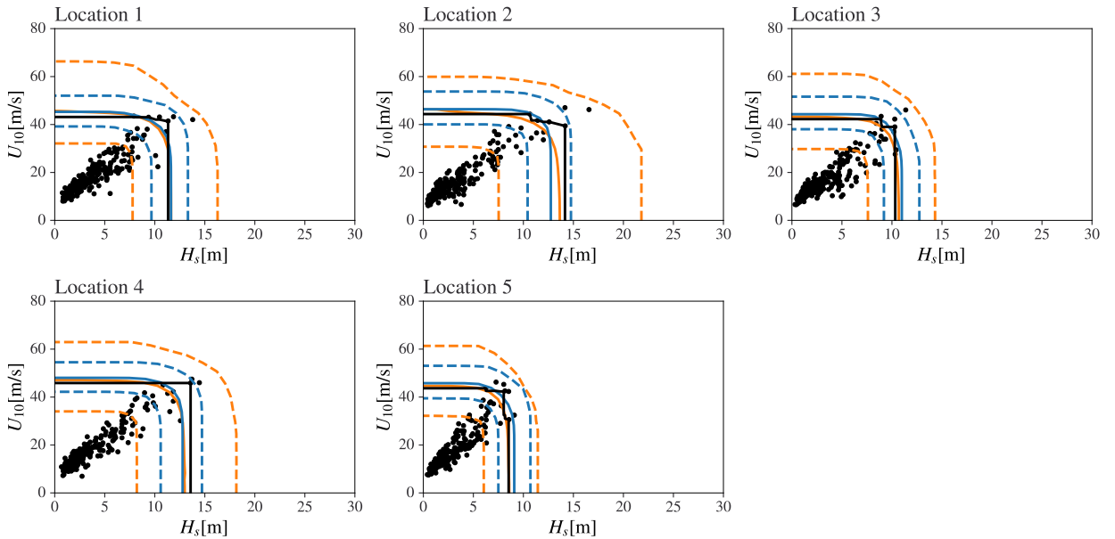
Figure S.6.4: Environmental contours of levels corresponding to 300 year return period for the west cluster. To be compared with fig. 9.
