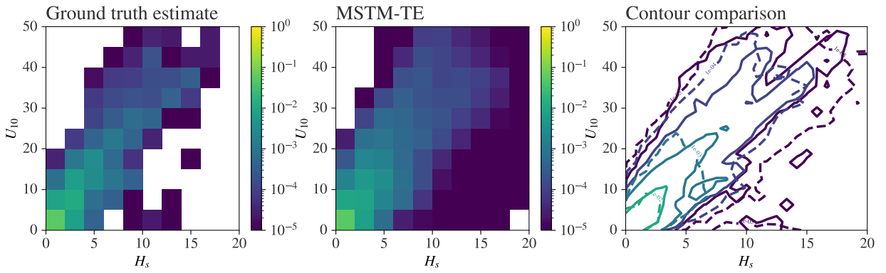
Figure S.8.4: (Location 4) The probability density of the original samples and the samples simulated using MSTM-TE
