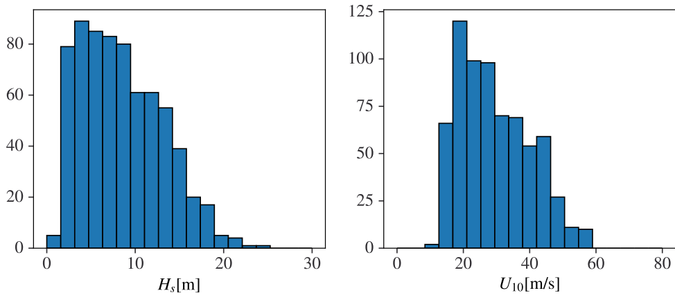
Figure S.2.2: Histogram of MSTM for the Guadeloupe region (60.5-62.5W°, 15.0N-17.0N°) illustrated in fig. 1
