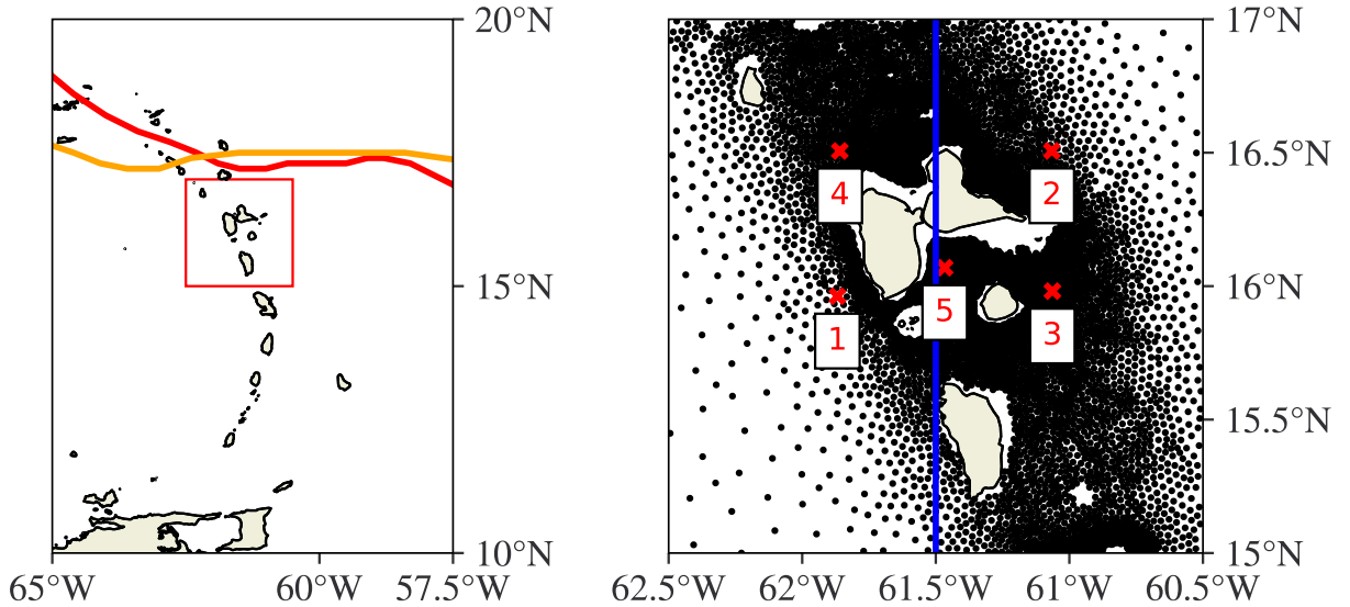
Figure 1: Leeward Islands and Guadeloupe. Left: the full spatial domain of the Leeward Islands (referred to for clarity as the Leeward region), with red box highlighting the Guadeloupe region of interest. Two tracks from cyclone events used for fig. 3 are also plotted; note that the Leeward region on which cyclones are simulated, is larger than the Guadeloupe region of interest in this work. Right: magnified view of the Guadeloupe region including the islands of Guadeloupe, with simulation grid locations (black dots) and five locations (red crosses) to be considered in detail. In order, the latitude-longitude coordinates of Locations 1 to 5 are (61.87W°,15.96N°), (61.07W°,16.51N°), (61.06W°,15.98N°), (61.86W°,16.51N°), (61.47W°,16.07N°). The vertical blue line at longitude 61.5W is used to partition the set of cyclones into west and east clusters.
