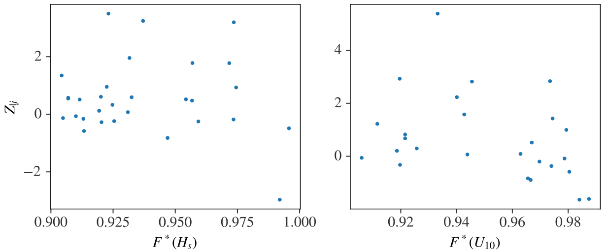
Figure S.3.11: Residual Z_{ij} calculated for the east cluster using inappropriate parameters (a, b) = (0.70, 0.50) for H_S and (0.80, -0.50) for U_{10} . The true estimated parameters were (0.29, -0.07) and (0.19, 0.36) respectively. The marginal threshold is 60% and the dependency threshold is 90% for this setting.
