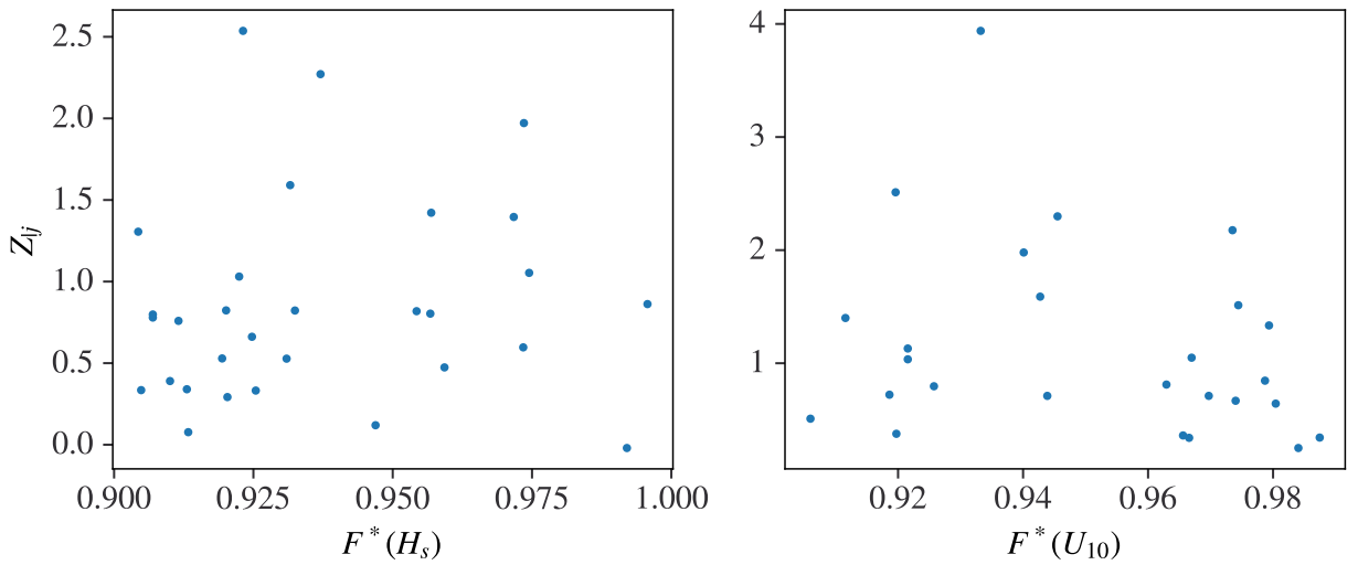
Figure S.3.9: Residual Z_{lj} against the conditioning variable (in uniform margins) for the east cluster.
