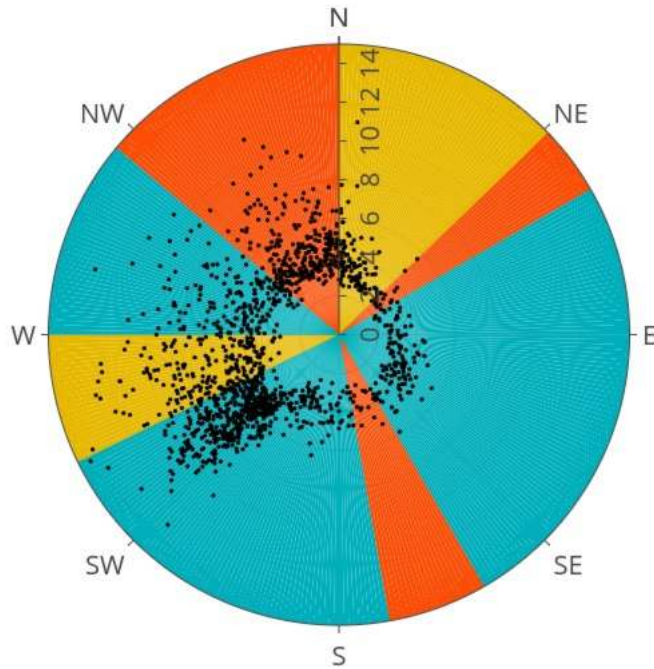
Figure 7: Polar plot showing combined deductions from tests of hypotheses for max-domain of attraction of H_S^{sp} at the \alpha = 5\% significance level. Orange: \xi(\theta) = 0, x^{F_\theta} = \infty ; yellow: \xi(\theta) = 0, x^{F_\theta} < \infty ; blue: \xi(\theta) < 0 . The original directional sample of H_S^{sp} on direction \theta is also shown as black dots.
