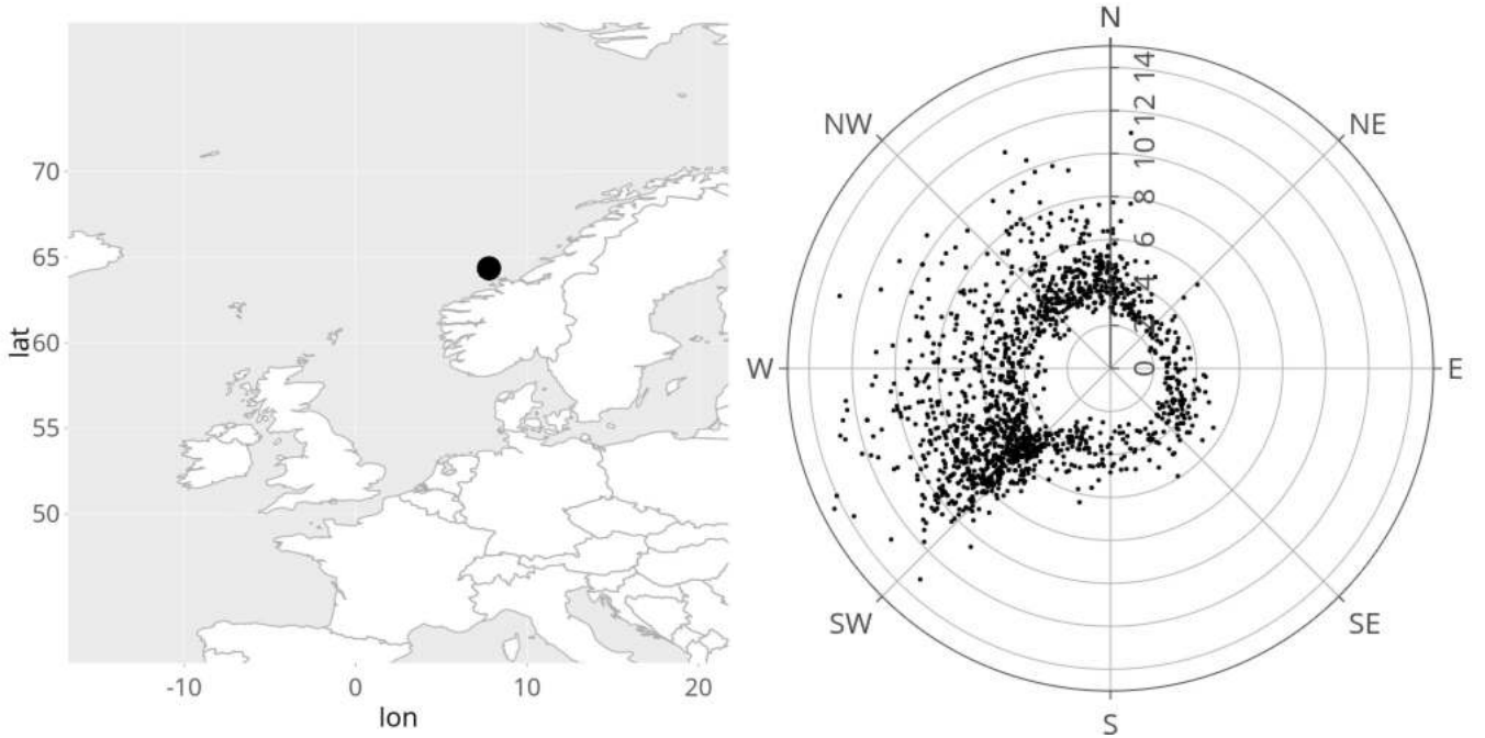
Figure 1: Left: map showing the North Sea location. Right: polar scatter-plot of H_S^{sp} on the direction \theta from which waves propagate; radial scale of H_S^{sp} is in metres.
