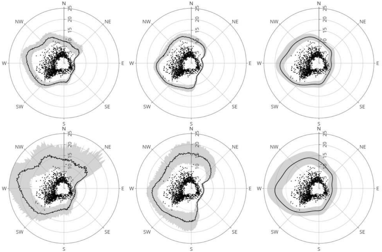
Figure 8: Rose diagrams for the 100-year (top) and 10,000-year (bottom) levels based on M ( left ), local ML ( middle ) and spline ML ( right ) estimators. Bootstrap means and corresponding 95% confidence bands are displayed as a function of direction measured clockwise from north.
