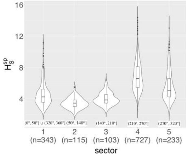
Figure 2: Violin plots of H_S^{sp} observations to the total of N = 1521 data points, with n here referring to the number of observations in each of the 5 sectors considered.
