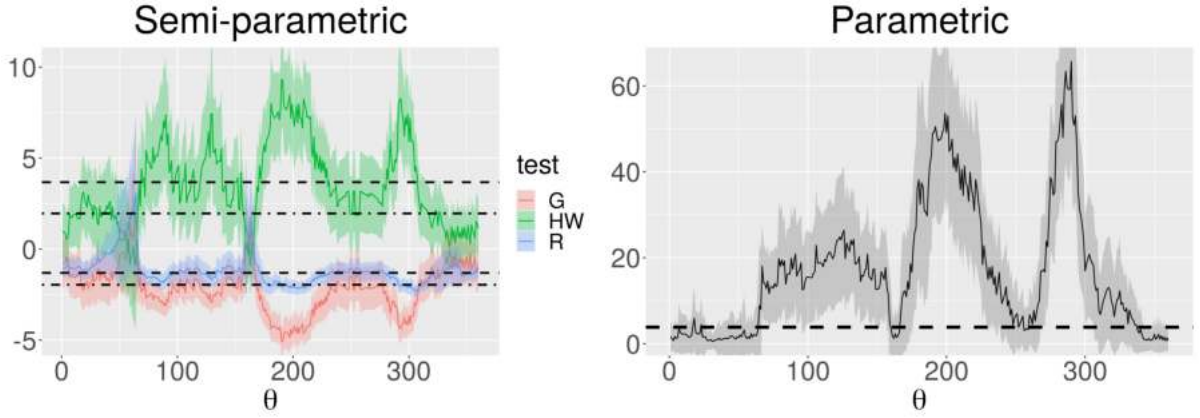
Figure 5: Bootstrap mean and corresponding 95% confidence intervals for the ratio ( R , R ), Greenwood-type ( G , G ) and Hasofer-Wang ( HW , W ) (left) and likelihood ratio ( LR , D ) (right) test statistics for \xi = 0 . Horizontal lines in both panels indicate asymptotic critical values at significance level \alpha = 5\% . In the left panel: dashed lines for R test ( -1.305 and 3.676 ); dot-dashed lines for G and W ( \pm 1.96 ). In the right panel: dashed line at 3.84 .
