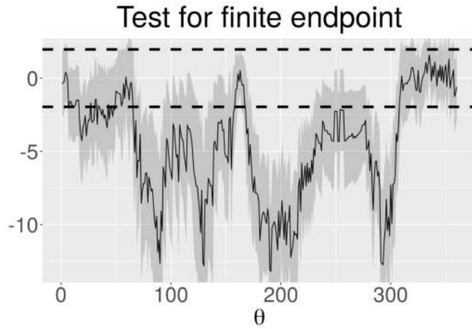
Figure 6: Bootstrap mean and corresponding 95% confidence intervals for the T-test statistic. The horizontal dashed lines correspond to the asymptotic critical values at the significance level \alpha = 5\% , i.e. the normal quantiles which are solutions of |z_\varepsilon| = 1.96 .
